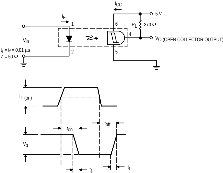
Figure 1. Switching Test Circuit
