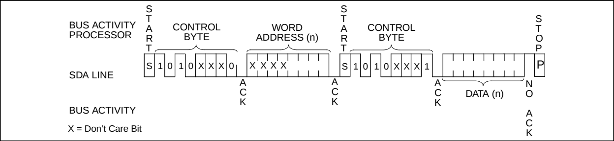
FIGURE 6-8: SEQUENTIAL READ
