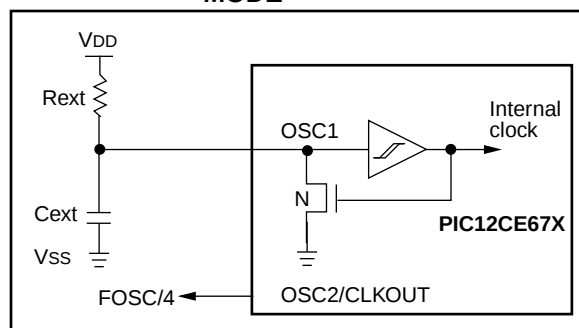
FIGURE 9-6: EXTERNAL RC OSCILLATOR MODE
