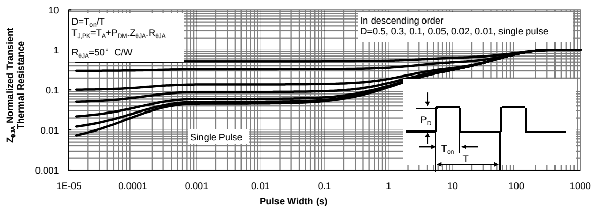
Pulse Width (s) Figure 16: Normalized Maximum Transient Thermal Impedance (Note H)
