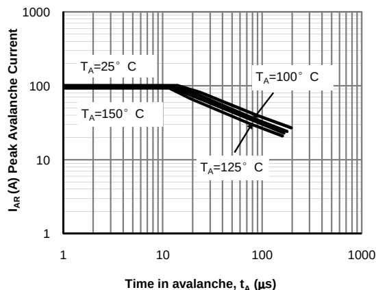
Time in avalanche, t_A ( \mu s) Figure 12: Single Pulse Avalanche capability (Note C)
