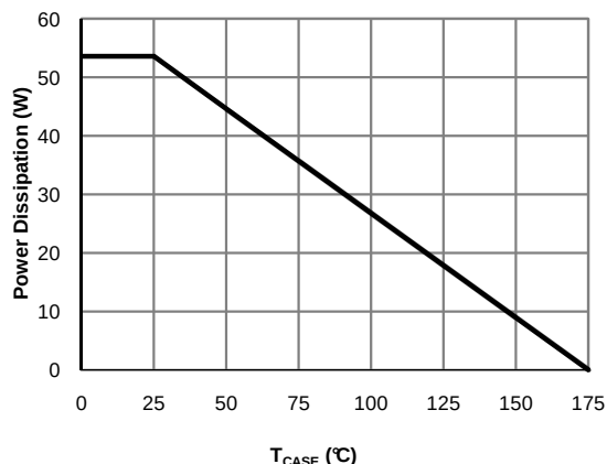
T_{CASE} ( ^{\circ} C) Figure 13: Power De-rating (Note F)
