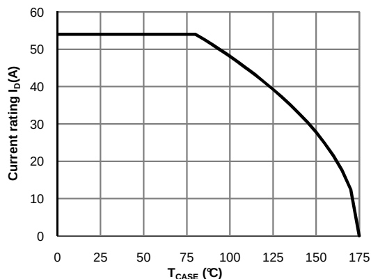
T_{CASE} ( ^{\circ} C) Figure 14: Current De-rating (Note F)
