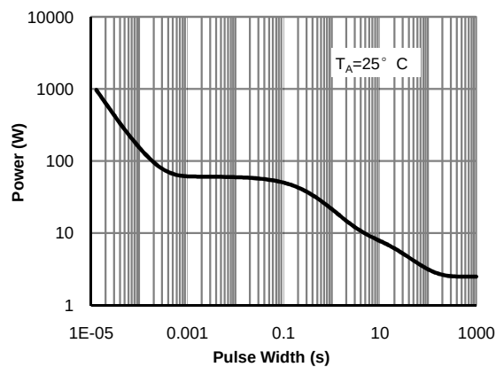
Pulse Width (s) Figure 15: Single Pulse Power Rating Junction-to-Ambient (Note H)
