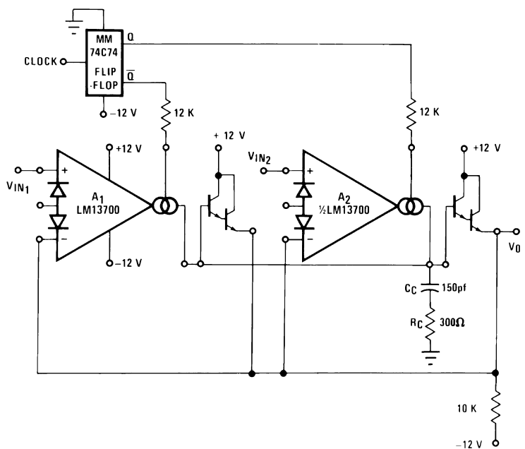
FIGURE 20. Multiplexer
