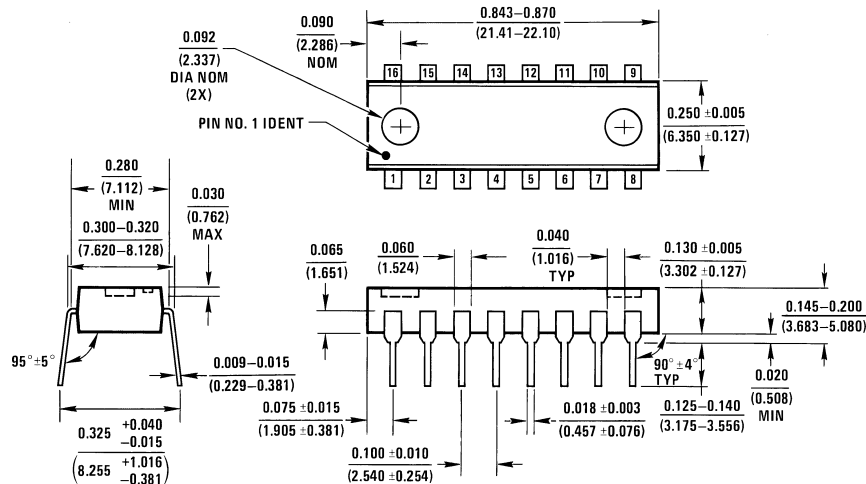
Molded Dual-In-Line Package (N) Order Number LM13700N or LM13700AN NS Package Number N16A
