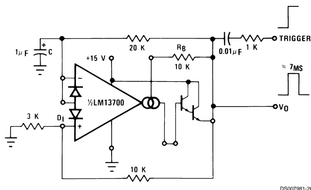
FIGURE 19. Zero Stand-By Power Timer
