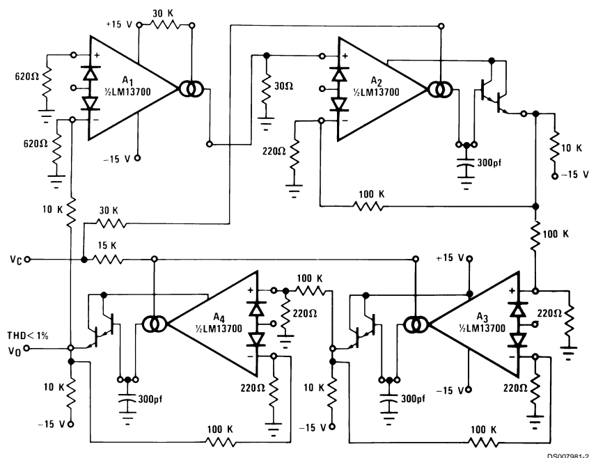
FIGURE 17. Sinusoidal VCO
