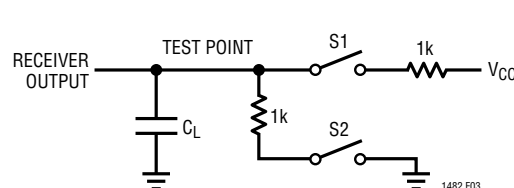
Figure 3. Receiver Timing Test Load
