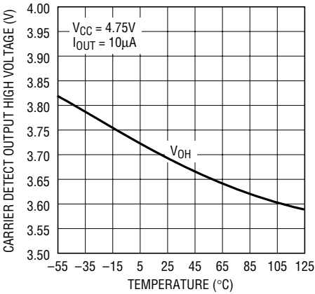
Carrier Detect Output High Voltage vs Temperature
