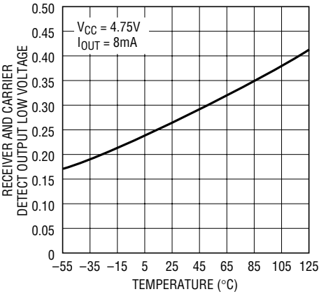
Receiver and Carrier Detect Output Low Voltage vs Temperature
