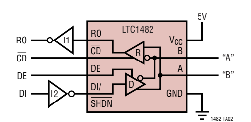
Fail-Safe “0” Application (Idle State = Logic “0”)
