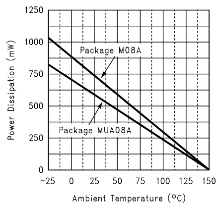
Power Derating Curves
