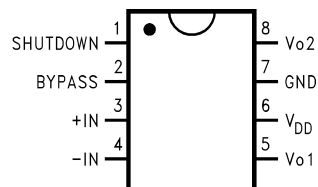
Small Outline (SO) Package
