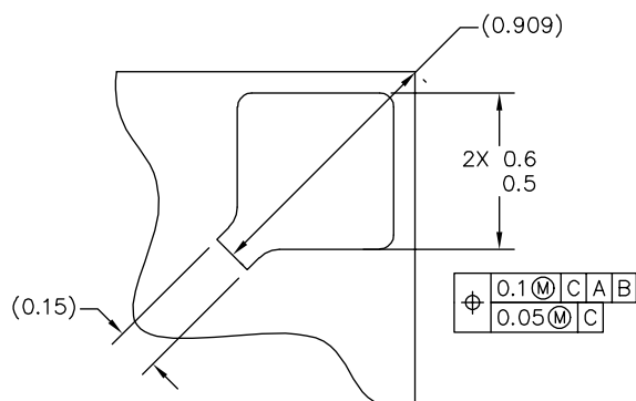
DETAIL T BACKSIDE PIN 1 INDEX
