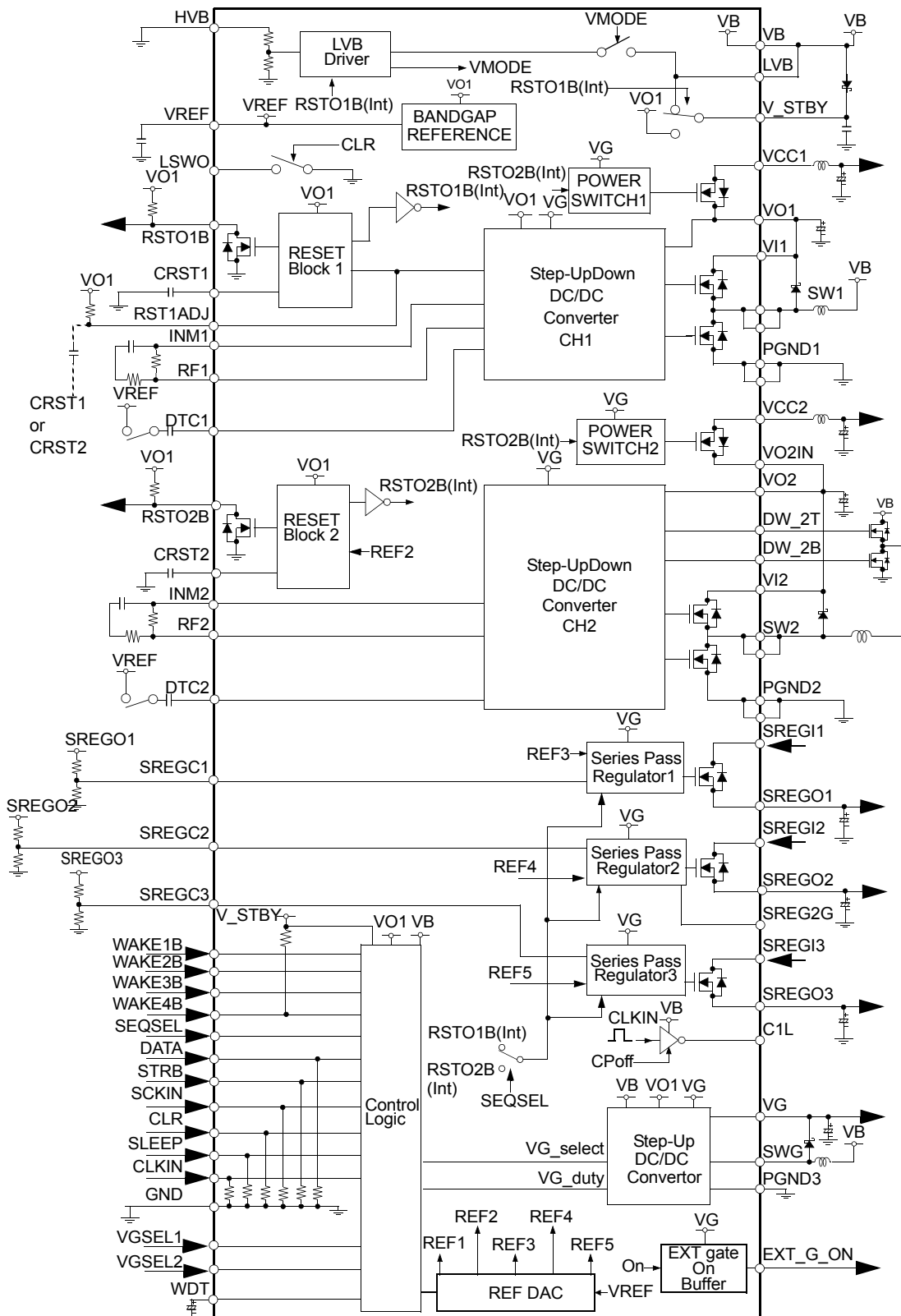
Figure 12. MPC18730 Typical Application Diagram (Ni-MH Battery)
