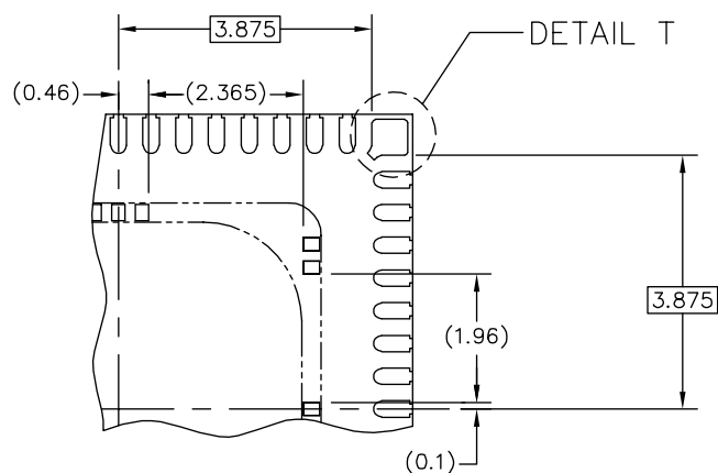
DETAIL M BACKSIDE PIN 1 INDEX
