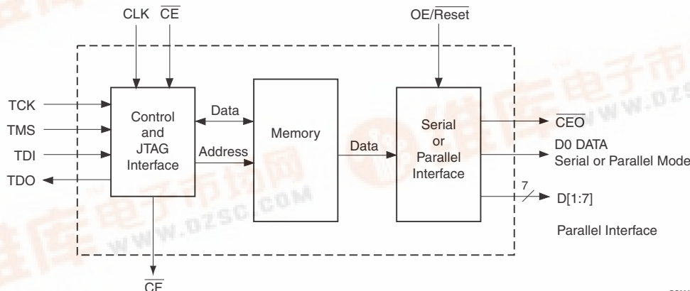
Figure 1: XC18V00 Series Block Diagram
