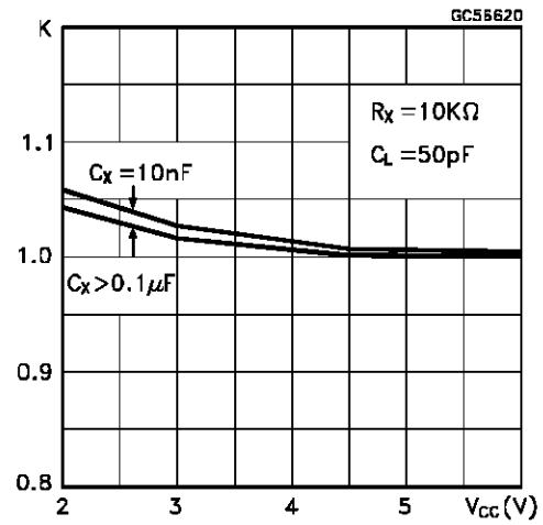
Output Pulse Width Constant Characteristics (for HC221A)
