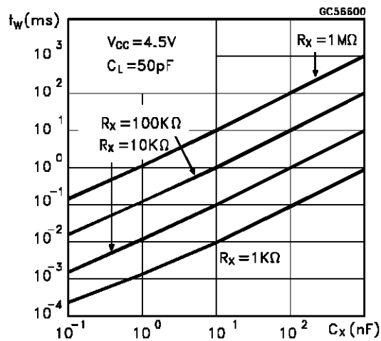
Output Pulse Width Characteristics (for HC221)
