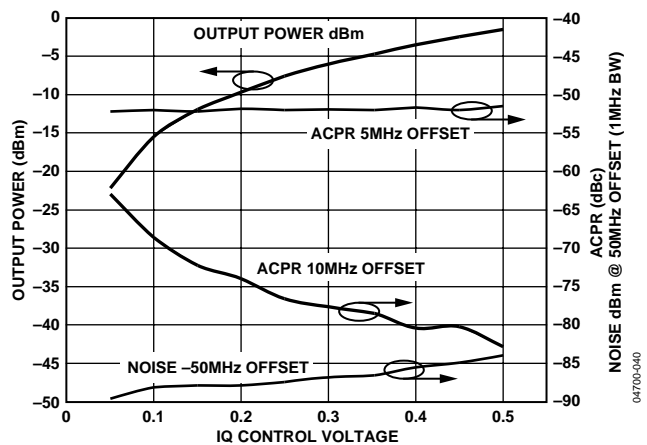
Figure 40. AD8341 Output Power, ACPR and Noise vs. V_{IQ} . Single-Carrier WCDMA (Test Model 1-64 at 2140 MHz)
