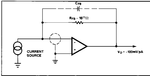
Figure 11. Pico Ammeter — The response time of this circuit is R_{FB} \times C_{FB} , where C_{FB} is the stray capacitance between the output and the inverting terminal of the amplifier.
