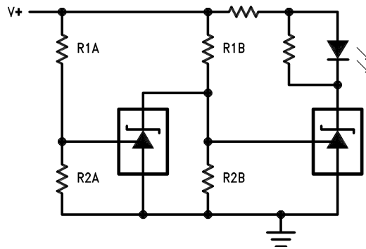
Voltage Monitor
