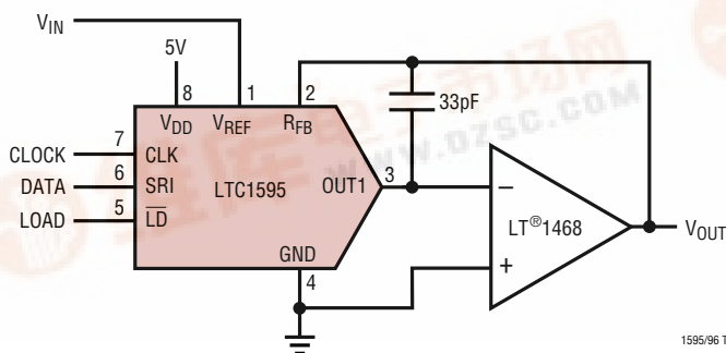
SO-8 Multiplying 16-Bit DAC Has Easy 3-Wire Serial Interface
