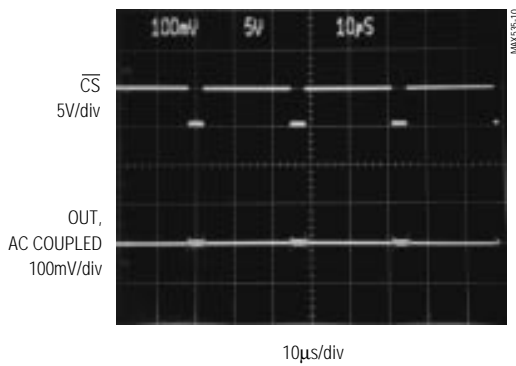
MAJOR-CARRY TRANSITION
