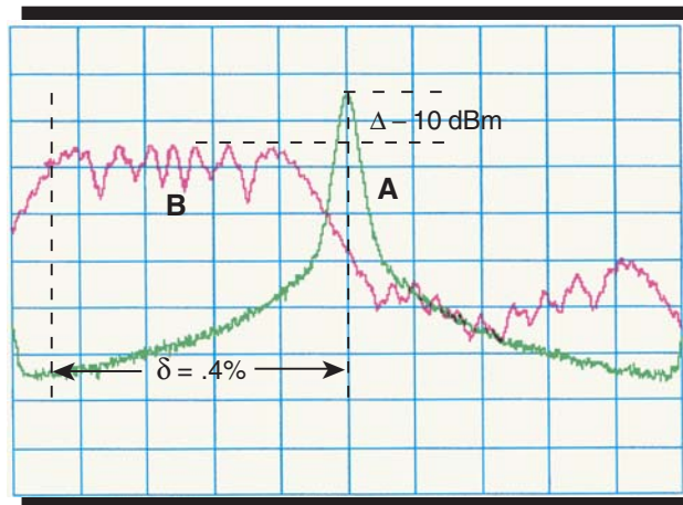
FIGURE 4B. 200MHz CLOCK OUTPUT IN FREQUENCY DOMAIN
