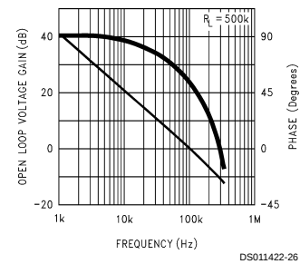
Gain and Phase Response vs Temperature ( -55^\circ C to +125^\circ C )
