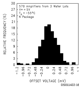
Distribution of LMC6061 Input Offset Voltage ( T_A = -55^\circ C )
