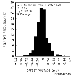
Distribution of LMC6061 Input Offset Voltage ( T_A = +25^\circ C )
