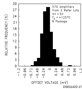
Distribution of LMC6061 Input Offset Voltage ( T_A = +125^\circ C )
