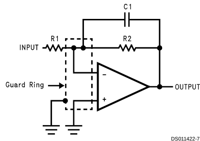
Inverting Amplifier
