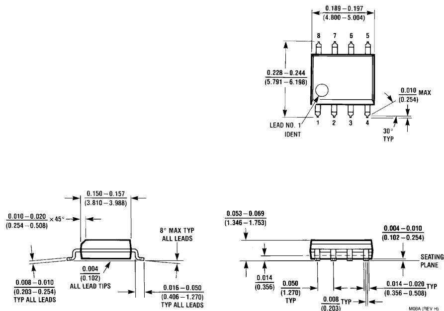
8-Pin Small Outline Package Order Number LMC6061AIM or LMC6061IM NS Package Number M08A
