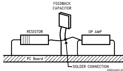
FIGURE 6. Air Wiring
