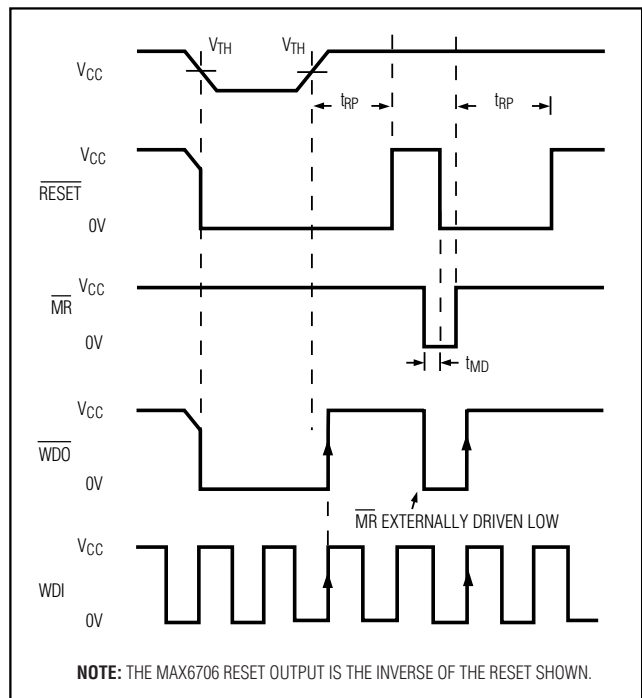
Figure 4. MAX6705/MAX6706/MAX6707 RESET, MR, WDO, and WDI Timing
