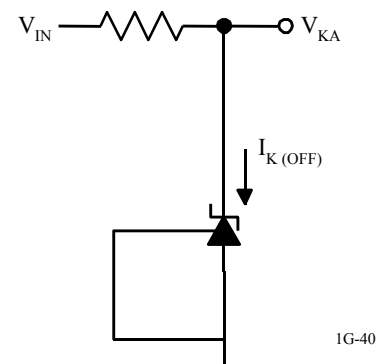
TEST CIRCUIT For I_{ROFF}
