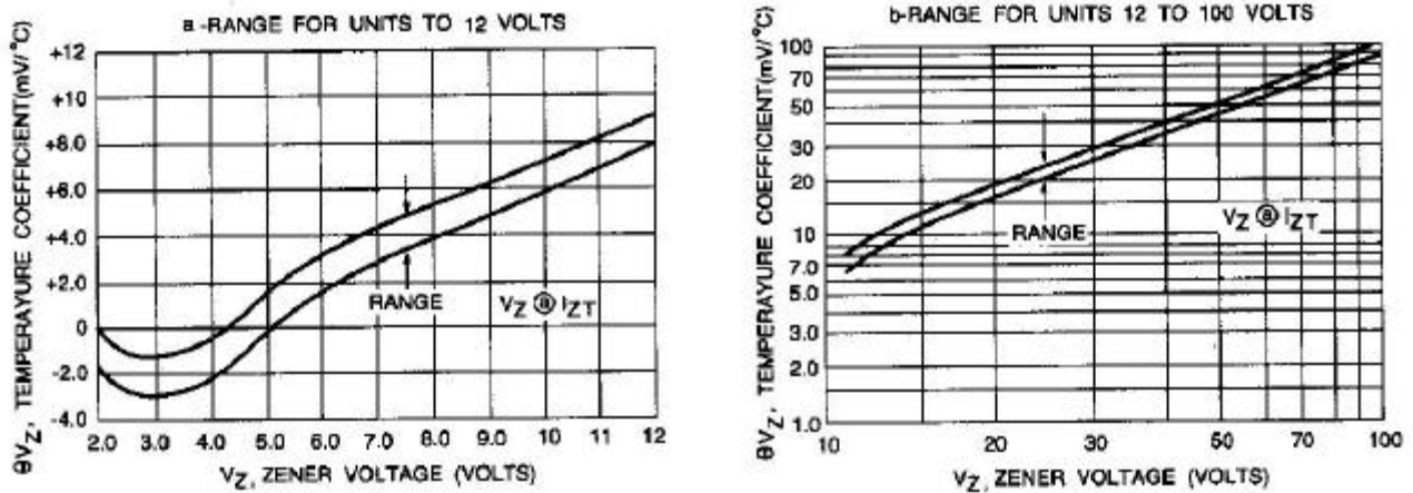
Fig. 2-TEMPERATURE COEFFICIENTS
