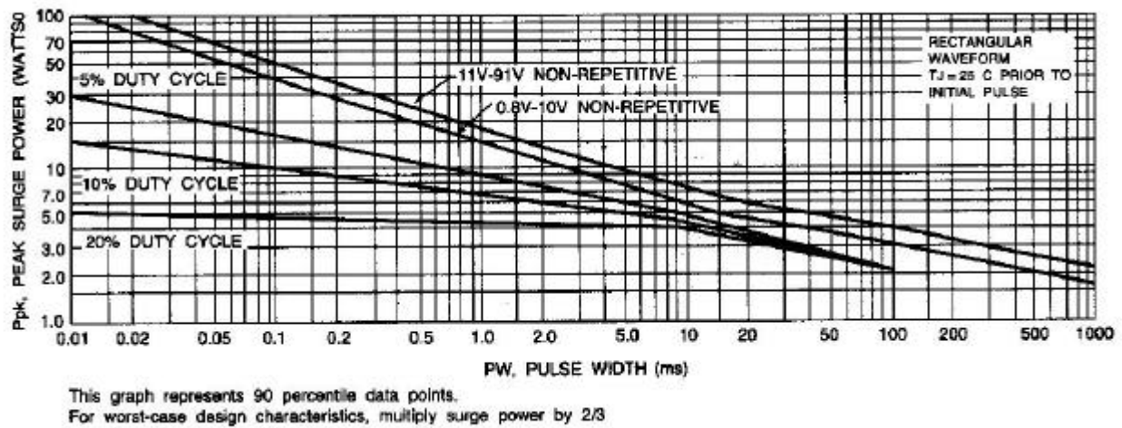
Fig. 5-MAXIMUM SURGE POWER
