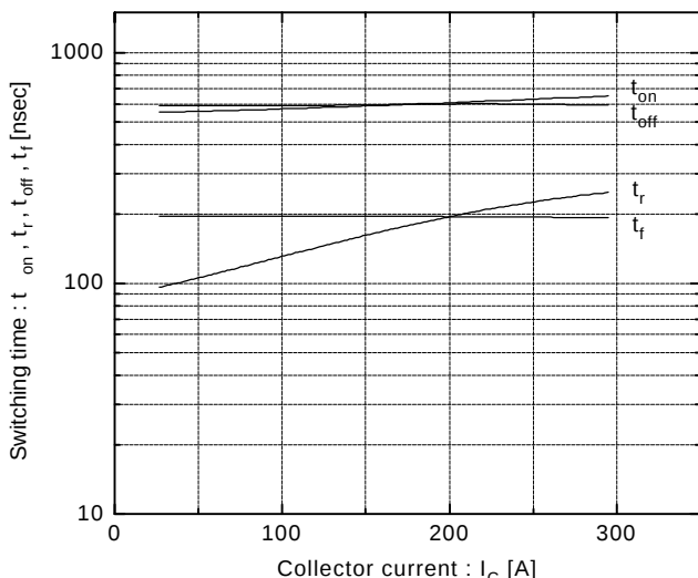
Switching time vs. Collector current V_{CC} = 300\text{V} , R_G = 9.1\Omega , V_{GE} = \pm 15\text{V} , T_J = 25^\circ\text{C}
