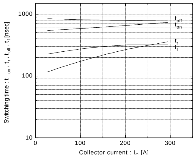
Switching time vs. Collector current V_{CC} = 300\text{V} , R_G = 9.1\Omega , V_{GE} = \pm 15\text{V} , T_J = 125^\circ\text{C}
