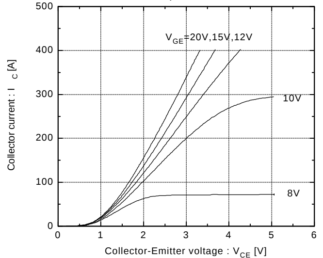
Collector current vs. Collector-Emittor voltage
