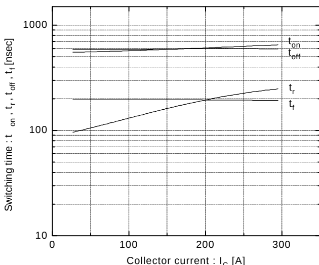
Switching time vs. Collector current V_{CC} = 300V, R_G = 9.1\Omega, V_{GE} = \pm 15V, T_J = 25^\circ\text{C}
