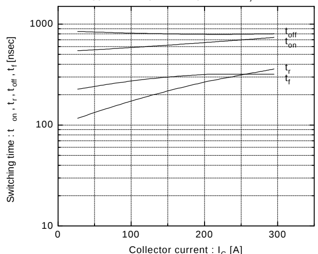
Switching time vs. Collector current V_{CC} = 300V, R_G = 9.1\Omega, V_{GE} = \pm 15V, T_J = 125^\circ\text{C}
