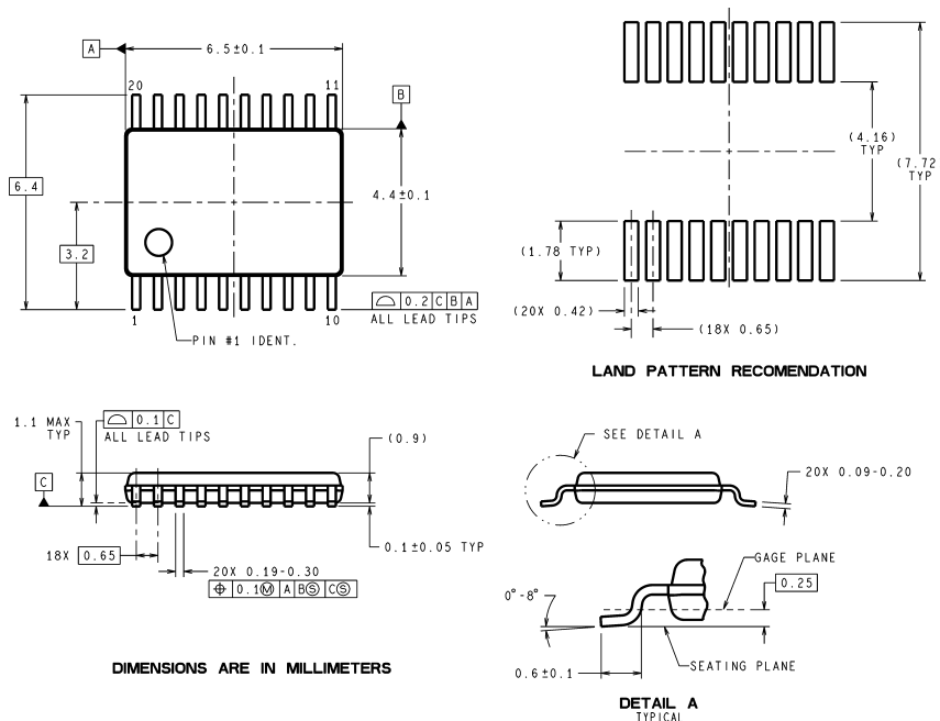
TSSOP-20 Pin Package (MTC) For Ordering, Refer to Ordering Information Table NS Package Number MTC20
