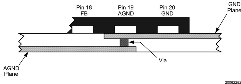
FIGURE 3. Multi-Layer Layout
