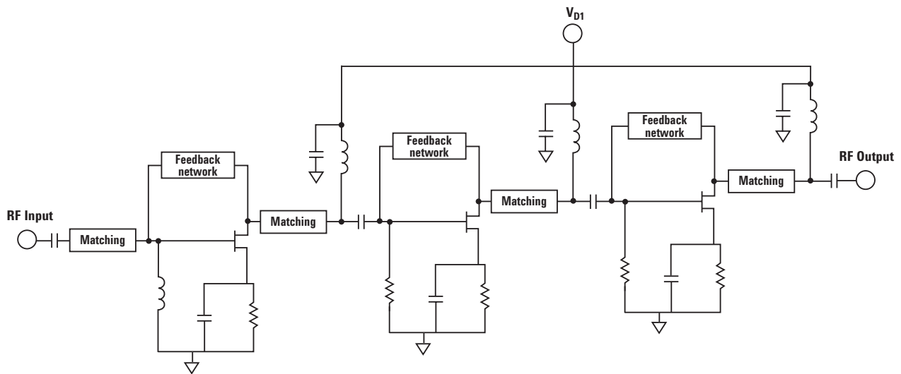
Figure 18. AMMC-5620 Schematic
