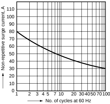
2-(1). Non-repetitive surge current vs. carrying time (AC output type)
