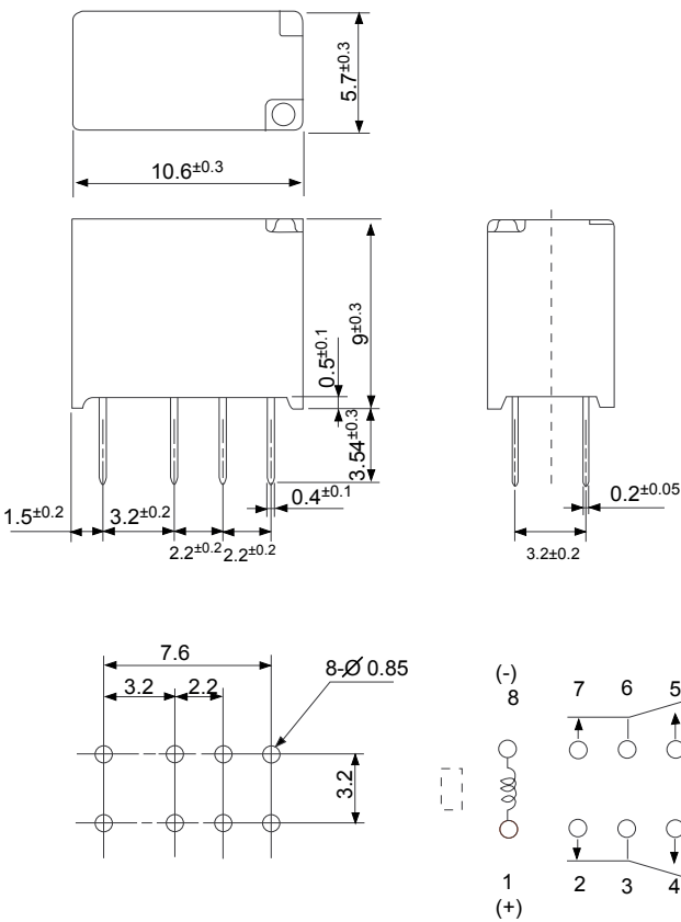
Recommended mounting pad (Tolerance: \pm 0.1 mm)
