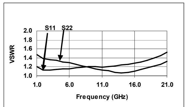
1 dB VSWR (S11, S22)
