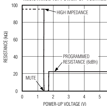
RESISTANCE vs. POWER-UP VOLTAGE
