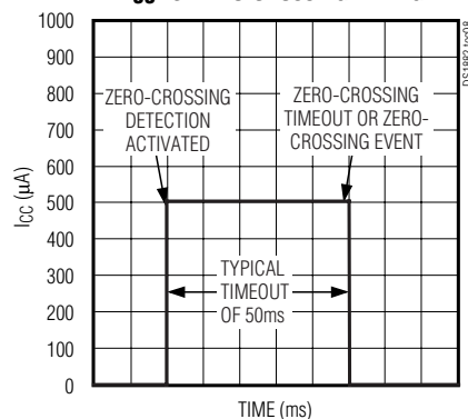
I_{CC} vs. ZERO-CROSSING TIMING
