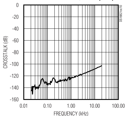
CROSSTALK vs. FREQUENCY (-6dB)
