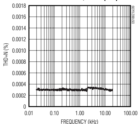
THD+N vs. FREQUENCY (0dB)
