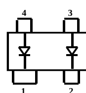
Unconnected Pair MA4E2054E-1068T
