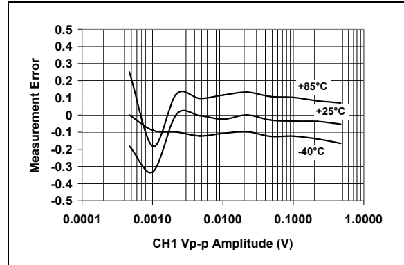
FIGURE 2-9: Measurement Error, Gain = 1, PF = + 0.5.
