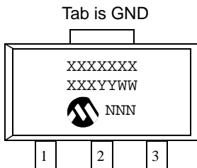
3-Lead SOT-223
