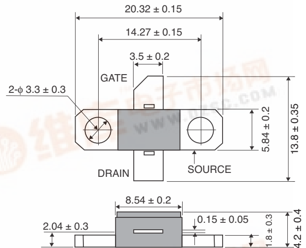
PACKAGE OUTLINE 3M
