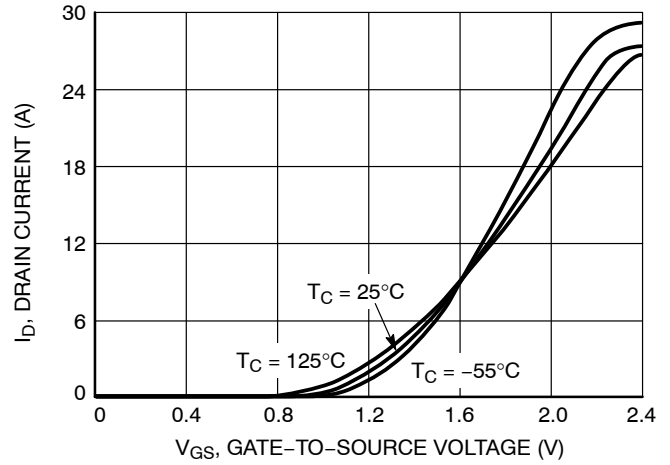
Figure 4. Transfer Characteristics
