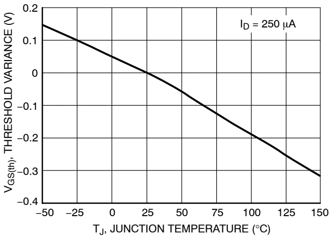
Figure 11. Threshold Voltage
