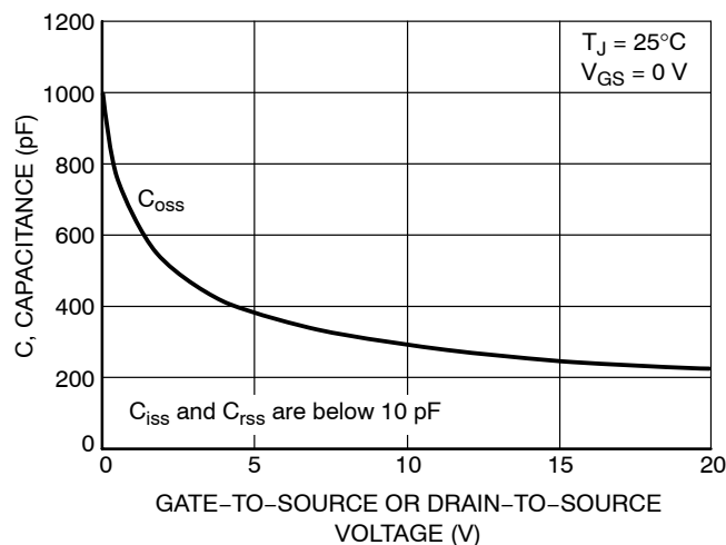
Figure 6. Capacitance Variation
