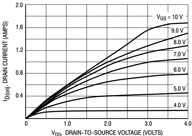
Figure 4. On-Region Characteristics
