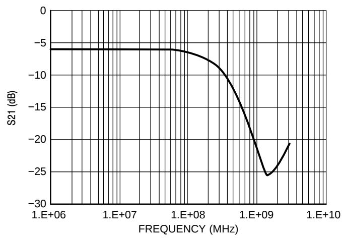
Figure 1. Insertion Loss Characteristic (50 \Omega Source and 50 \Omega Load Termination)
