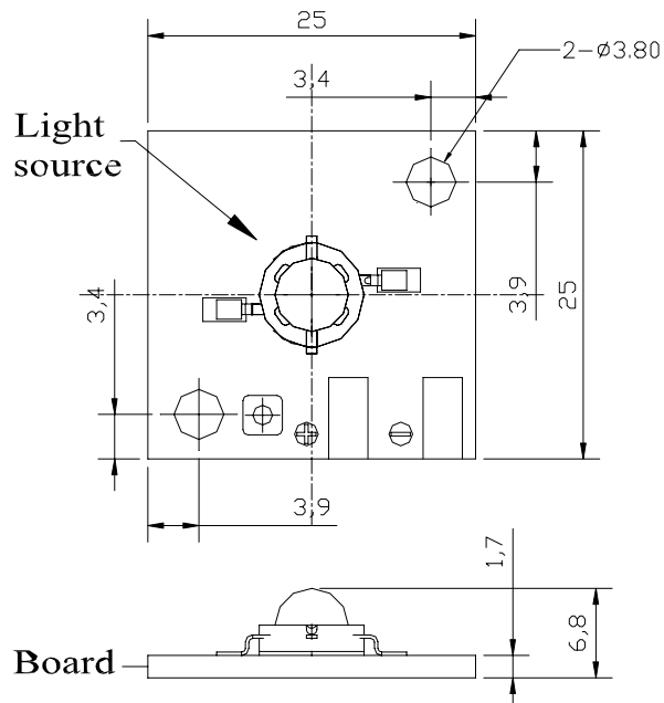
CMDA50xx15D13L Square Configuration
