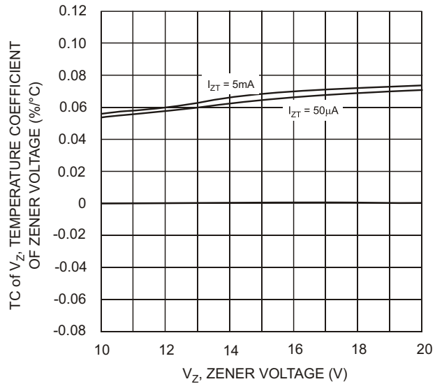
Fig. 17 Typical Temperature Coefficient of Zener Voltage vs. Zener Voltage, DDZX9697TS - DDZX9707TS
