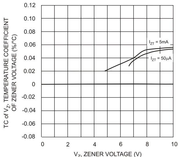
Fig. 16 Typical Temperature Coefficient of Zener Voltage vs. Zener Voltage, DDZX9692TS - DDZX9697TS
