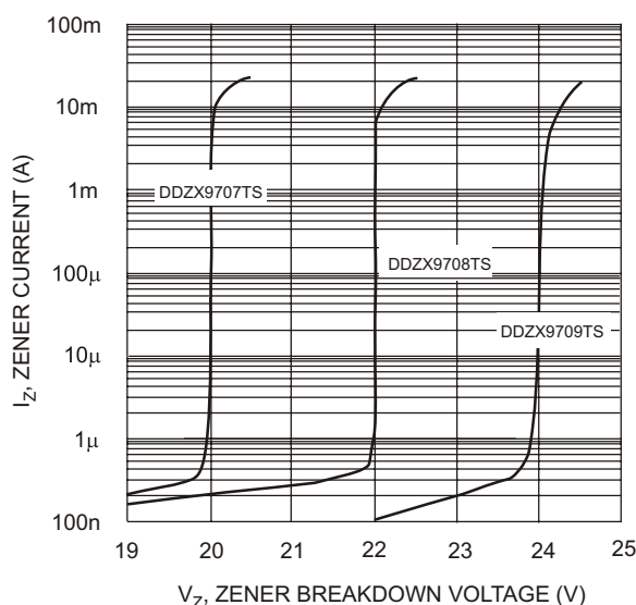
Fig. 7 Typical Reverse Characteristics, DDZX9707TS - DDZX9709TS
