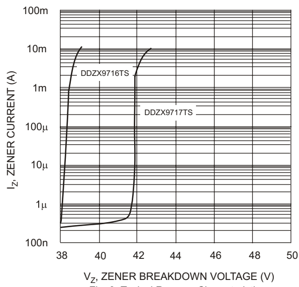
Fig. 9 Typical Reverse Characteristics, DDZX9716TS - DDZX9717TS
