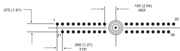
38 Contacts
