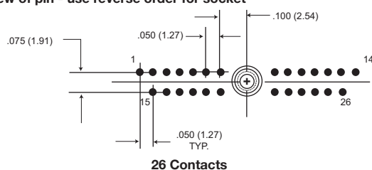
26 Contacts
