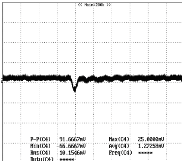
Figure 9: Output voltage response to step-change in load current (50%-75% of I_o , max; di/dt = 0.1A/\mu s ). Load cap: 10\mu F , tantalum capacitor and 1\mu F ceramic capacitor. Trace: V_{out} (50mV/div, 100us/div), Scope measurement should be made using a BNC cable (length shorter than 20 inches). Position the load between 51 mm to 76 mm (2 inches to 3 inches) from the module..
