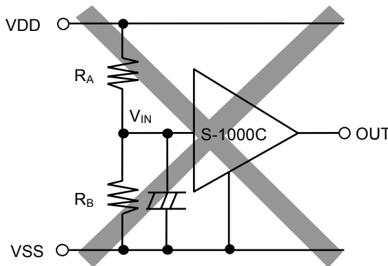
Figure 20 An example for bad implementation of input voltage divider
