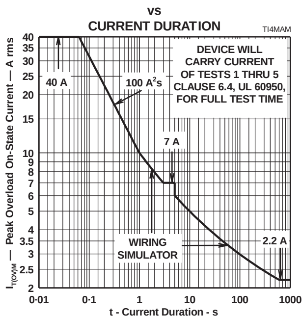
Figure 10. Peak Overload On-State Current against Duration
