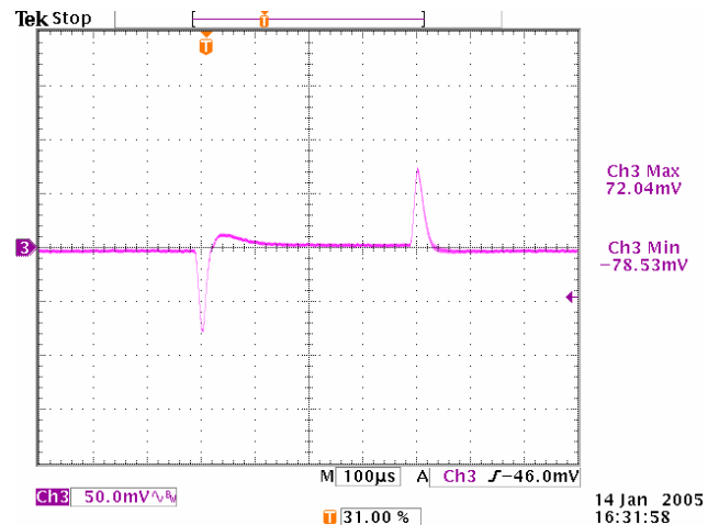
Figure 21. Vin=5V, Vout=1V, BW~40kHz
