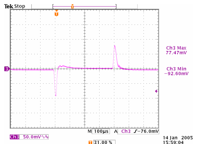
Figure 22. Vin=3.3V, Vout=1V, BW~40kHz
