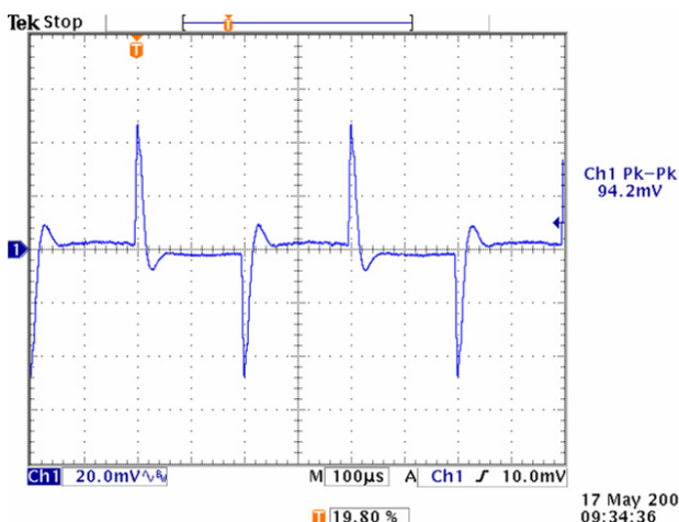
Figure 30. Transient Response without Optimal Voltage Positioning
