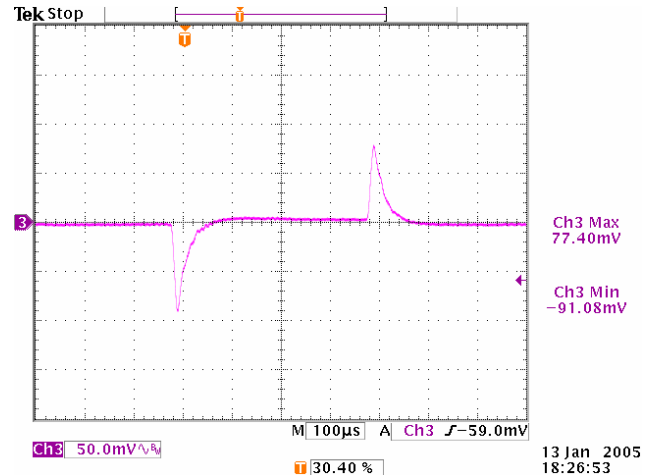
Figure 20. Vin=5V, Vout=2.5V, BW~45kHz
