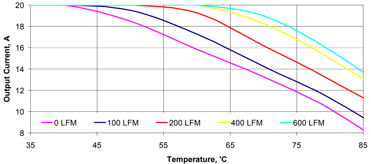
Figure 23. Thermal Derating Curves. V_{in}=13.2V , V_{out}=5.0V , F_{sw}=500kHz
