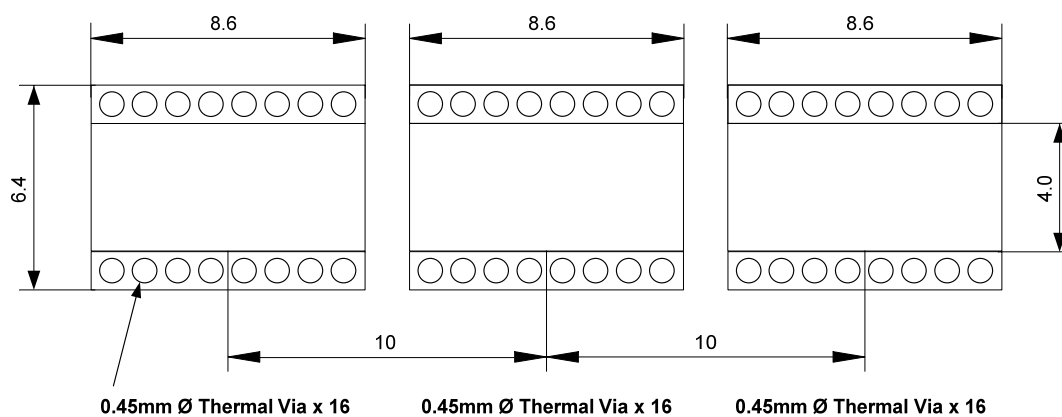
Figure 60. Recommended Pad Sizes
