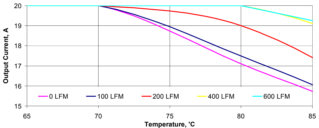
Figure 24. Thermal Derating Curves. V_{in}=5.0V , V_{out}=2.5V , F_{sw}=500kHz
