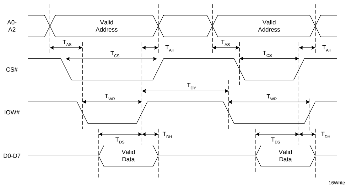
FIGURE 18. 16 MODE (INTEL) DATA BUS WRITE TIMING
