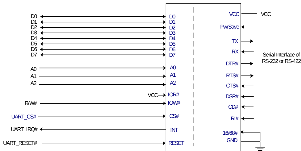
Motorola Data Bus Interconnections
