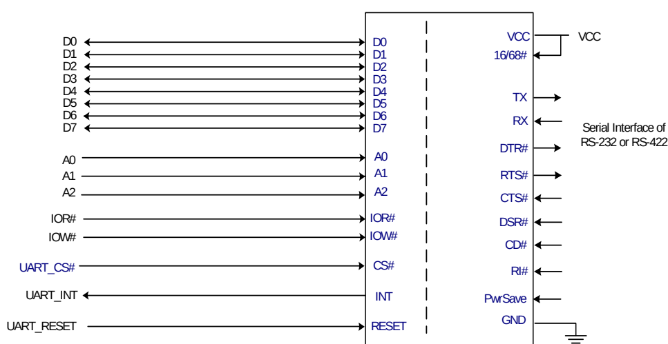
Intel Data Bus Interconnections
