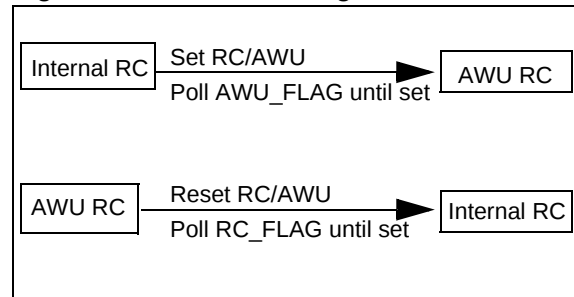
Figure 13. Clock Switching
