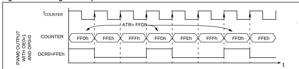
Figure 39. PWM Signal Example
