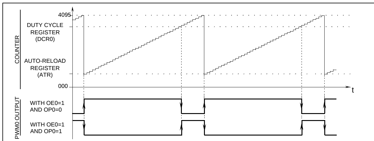
Figure 38. PWM Function
