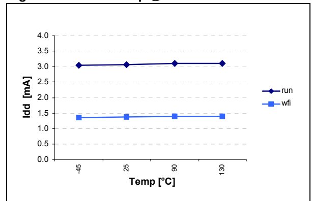
Figure 51. I_{DD} vs temp @V DD 5V & int RC=2MHz
