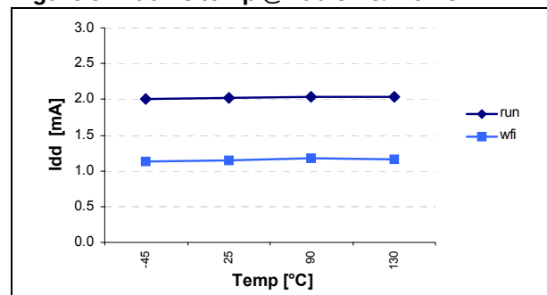
Figure 51. I_{DD} vs temp @V DD 5V & int RC=2MHz
