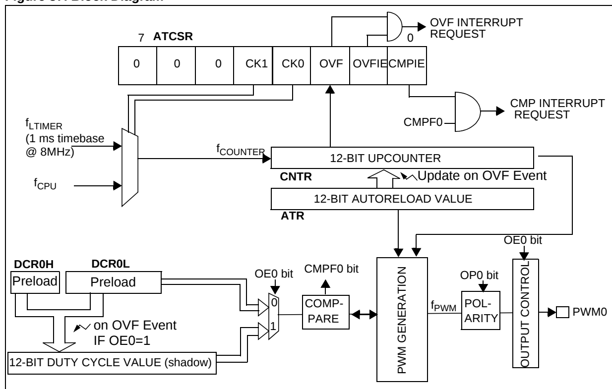
Figure 37. Block Diagram
