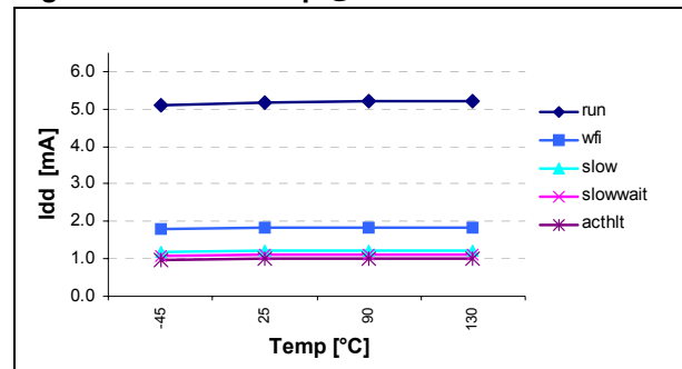
Figure 50. I_{DD} vs temp @V DD 5V & int RC=4MHz
