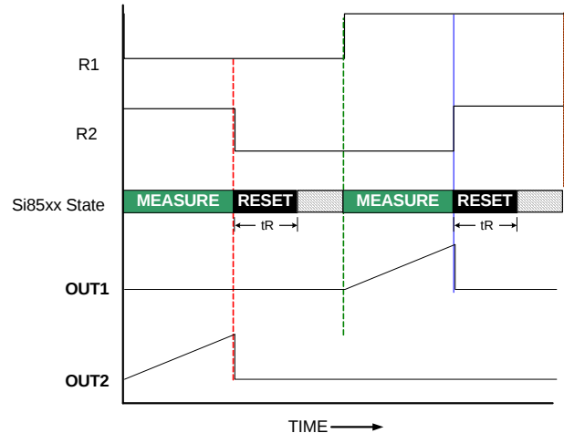
Figure 9. Full-Bridge Timing Example A
