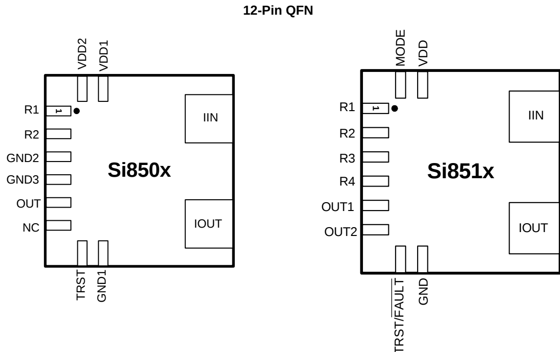
Figure 17. Example Pin Configurations
