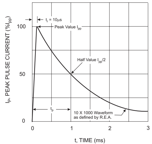
Fig. 4 Pulse Waveform
