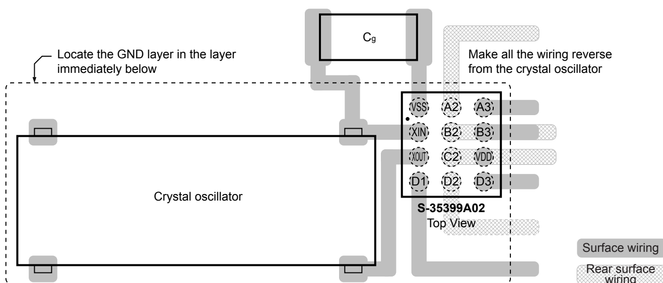
Figure 61 Connection Diagram 2
