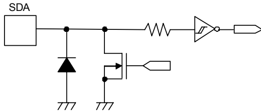
Figure 3 SDA Pin
