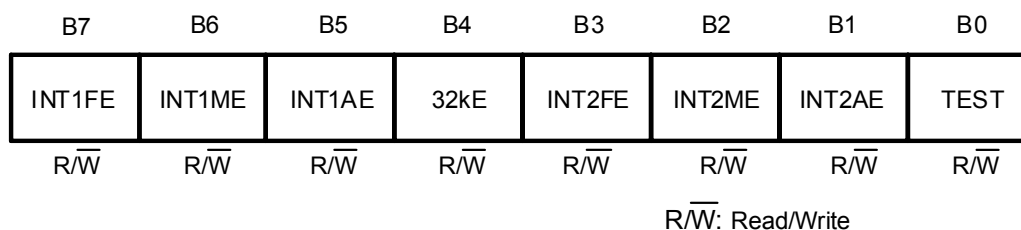
Figure 14 Status Register 2
