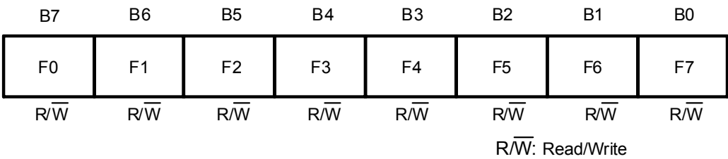
Figure 20 Free Register
