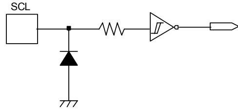
Figure 4 SCL Pin
