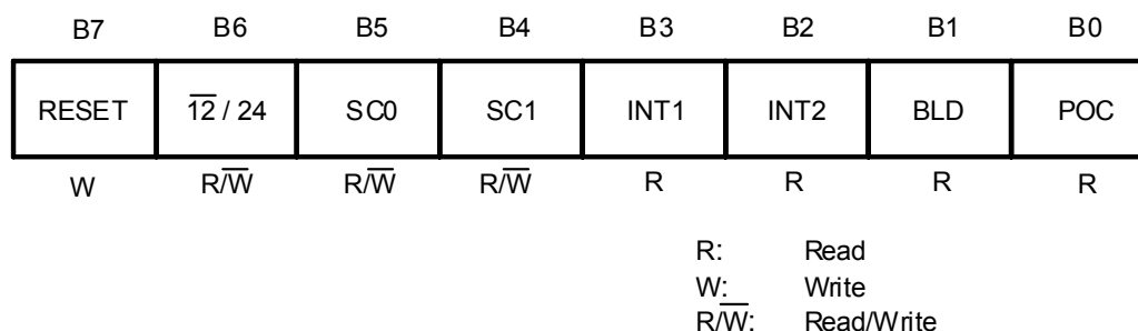
Figure 13 Status Register 1
