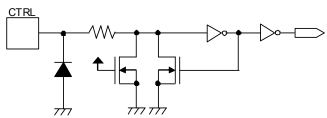
Figure 6 CTRL Pin
