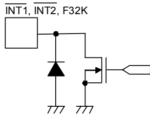
Figure 5 \overline{\text{INT1}} Pin, \overline{\text{INT2}} Pin, F32K Pin
