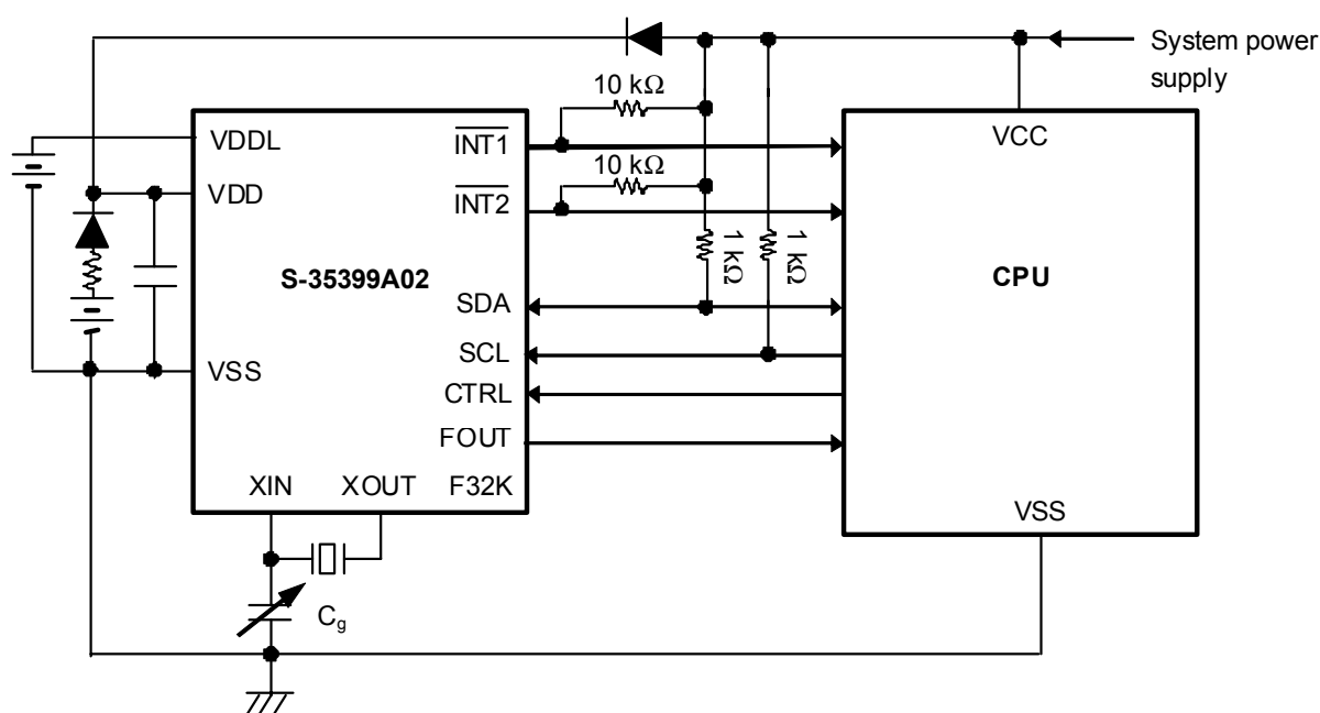
Figure 58 Application Circuit 1
