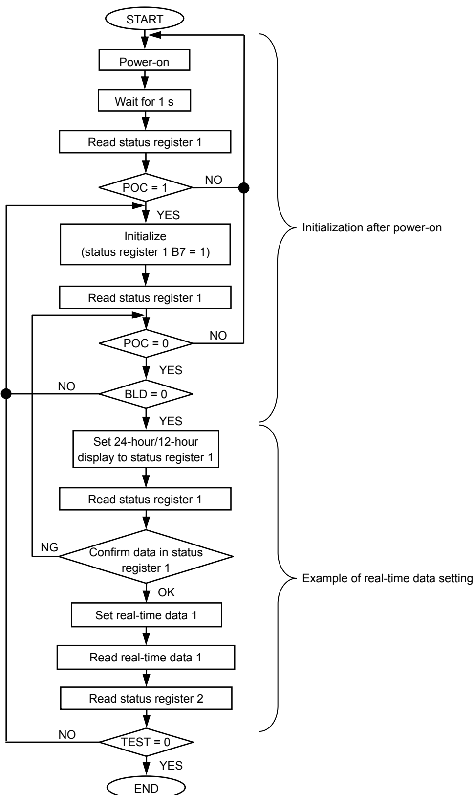
Figure 57 Example of Initialization Flowchart
