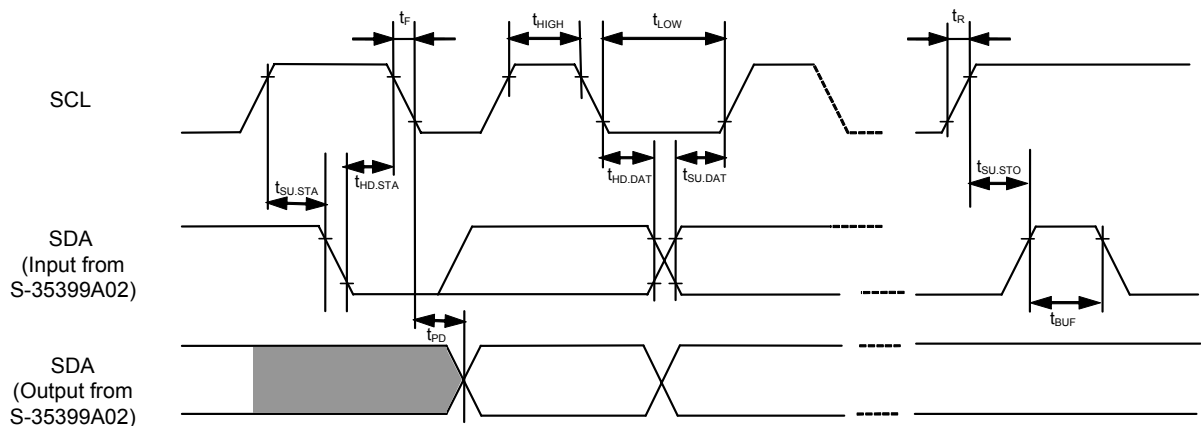
Figure 10 Bus Timing
