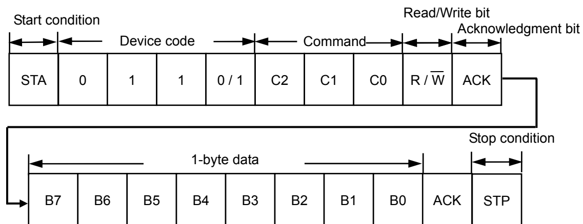
Figure 11 Data Communication
