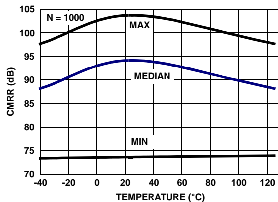
FIGURE 30. ISL28197 CMRR vs TEMPERATURE, V_{CM} = 0.5V TO 3.5V , V_+ , V_- = \pm 2.5V
