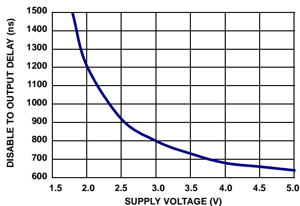
FIGURE 18. ISL28197 ENABLE LOW TO OUTPUT TURN-OFF TIME vs SUPPLY VOLTAGE
