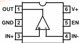
ISL28196, ISL28197 (6 LD SOT-23) TOP VIEW
