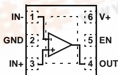
ISL28196, ISL28197 (6 LD 1.6X1.6X0.5 µTDFN) TOP VIEW
