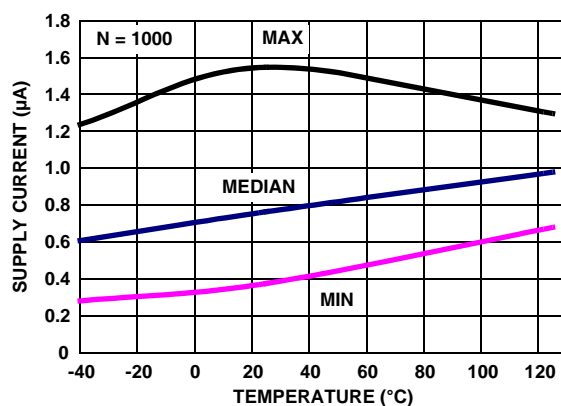
FIGURE 20. ISL28197 SUPPLY CURRENT vs TEMPERATURE, V_+ , V_- = \pm 2.5V
