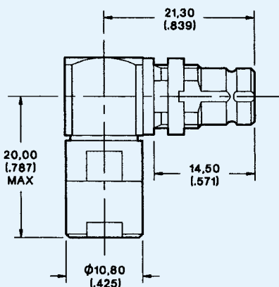
Mounting Plan BB (Page 109). Maximum Panel Thickness 2,00 (.078). Assembly Instruction BBAI-1231*
