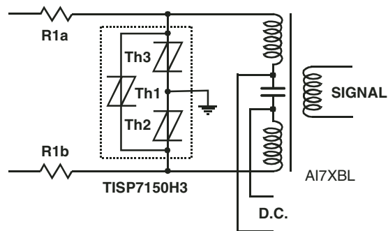
Figure 13. ISDN Protection
