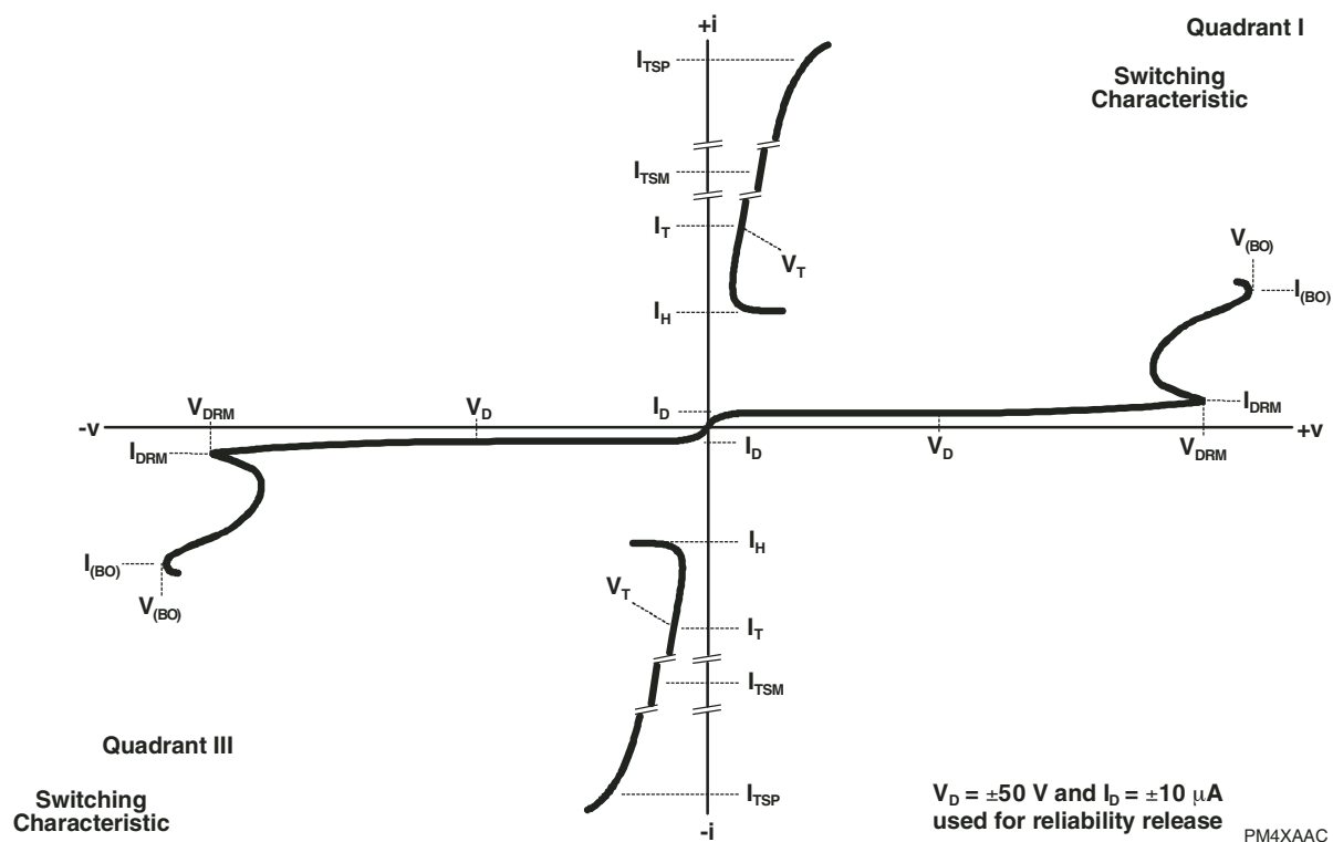
Figure 1. Voltage-current Characteristic for Terminal Pairs
