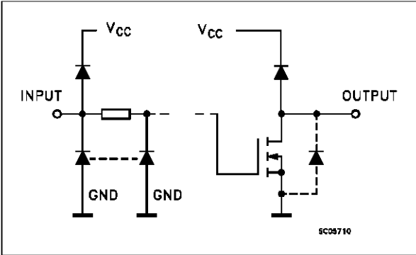
INPUT AND OUTPUT EQUIVALENT CIRCUIT (OPEN DRAIN OUTPUT, HC292/294)
