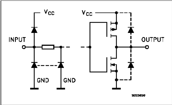
INPUT AND OUTPUT EQUIVALENT CIRCUIT (TOTEM POLE OUTPUT)
